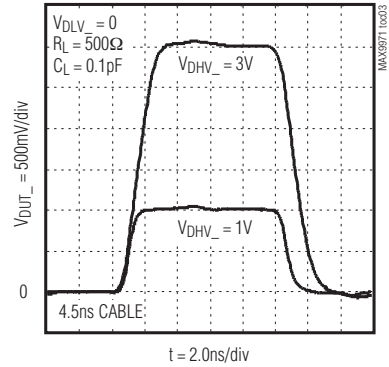
DRIVER LARGE-SIGNAL RESPONSE INTO 500Ω
